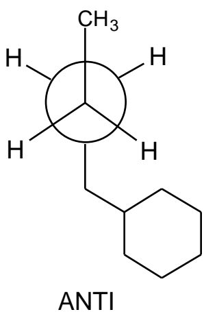
1-Cyclohexylbutane C2 - C3
