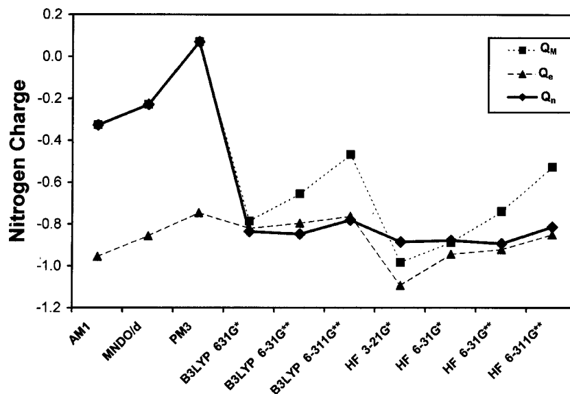
FIGURE 1. Variations in the Mulliken charge Q_M , the electrostatic charge Q_e , and the natural charge Q_n values when calculated at different levels of theory.
