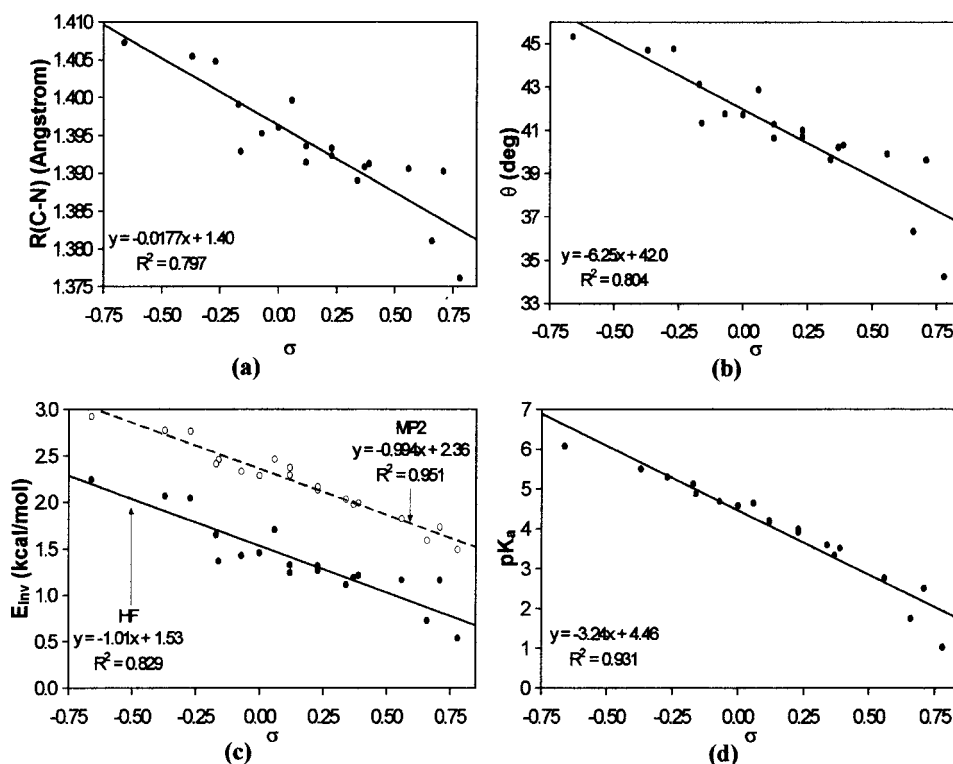
FIGURE 2. Correlations of the properties examined with the Hammett \sigma constants of the substituents: (a) The amino group C—N bond distance vs. \sigma , (b) the out-of-plane angle \theta vs. \sigma , (c) the inversion barriers E(\text{HF})_{\text{inv}} and E(\text{MP2})_{\text{inv}} vs. \sigma , and (d) the amino group pK_a vs. \sigma .
