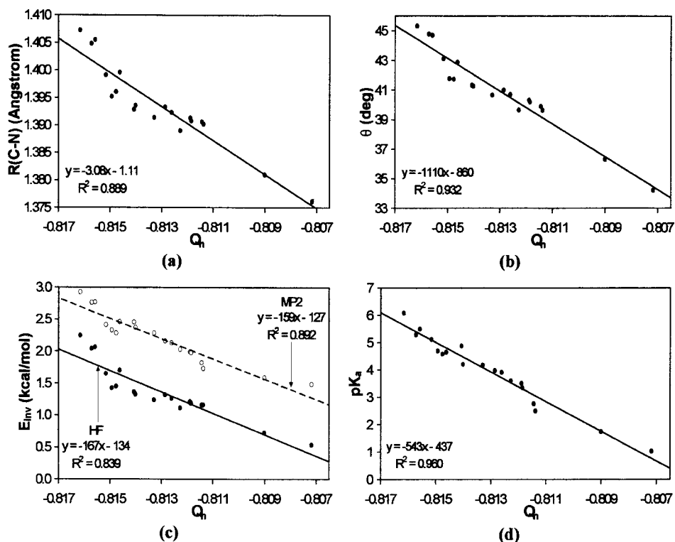
FIGURE 3. Correlations of the properties examined with the amino nitrogen atom natural charge Q_n : (a) The amino group C—N bond distance vs. Q_n , (b) the out-of-plane angle \theta vs. Q_n , (c) the inversion barriers E(\text{HF})_{\text{inv}} and E(\text{MP2})_{\text{inv}} vs. Q_n , and (d) the amino group pK_a vs. Q_n .
